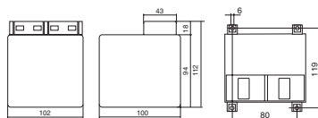
TARS3
