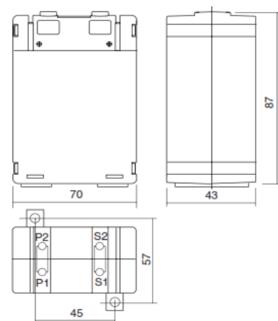
Accessori / Accessories
