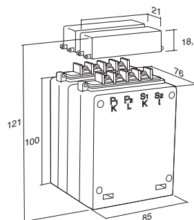
TARS4
