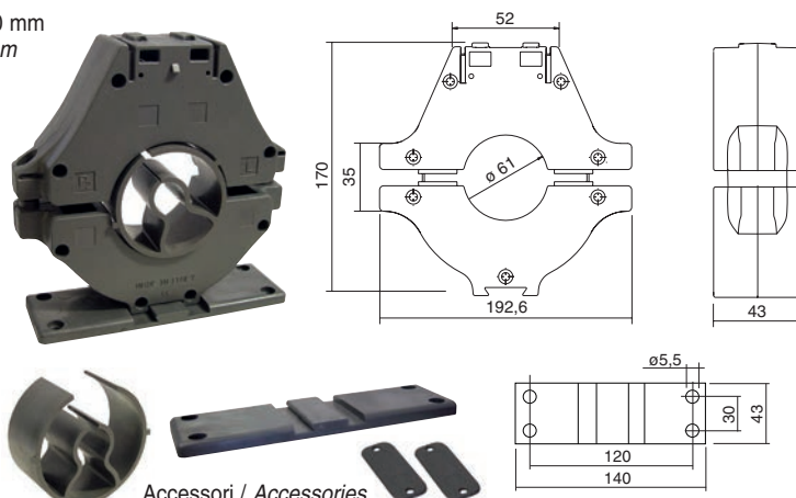
Accessori / Accessories
