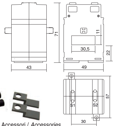
Accessori / Accessories
