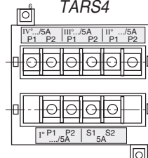
TARS4
