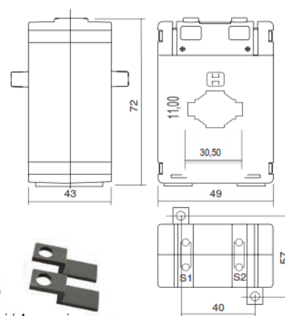
Accessori / Accessories
