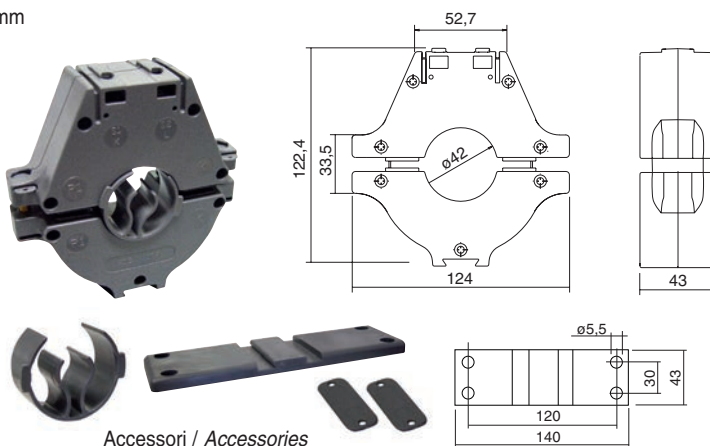
Accessori / Accessories
